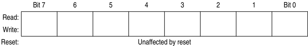
Figure 6-2. Accumulator (A)
