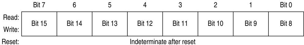
Figure 17-12. TIM2 Channel x Register High (T2CHxH)
